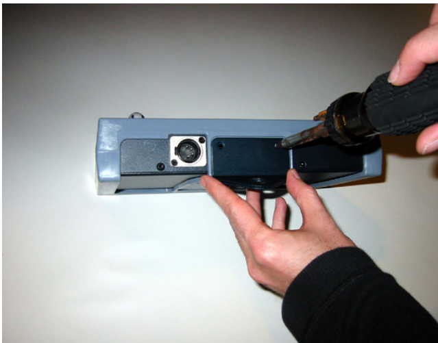
Attaching the small mounting bracket to the back of a PQ Controller
